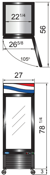
MCF8722GR
