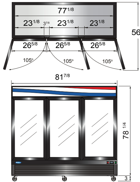
MCF8724GR
